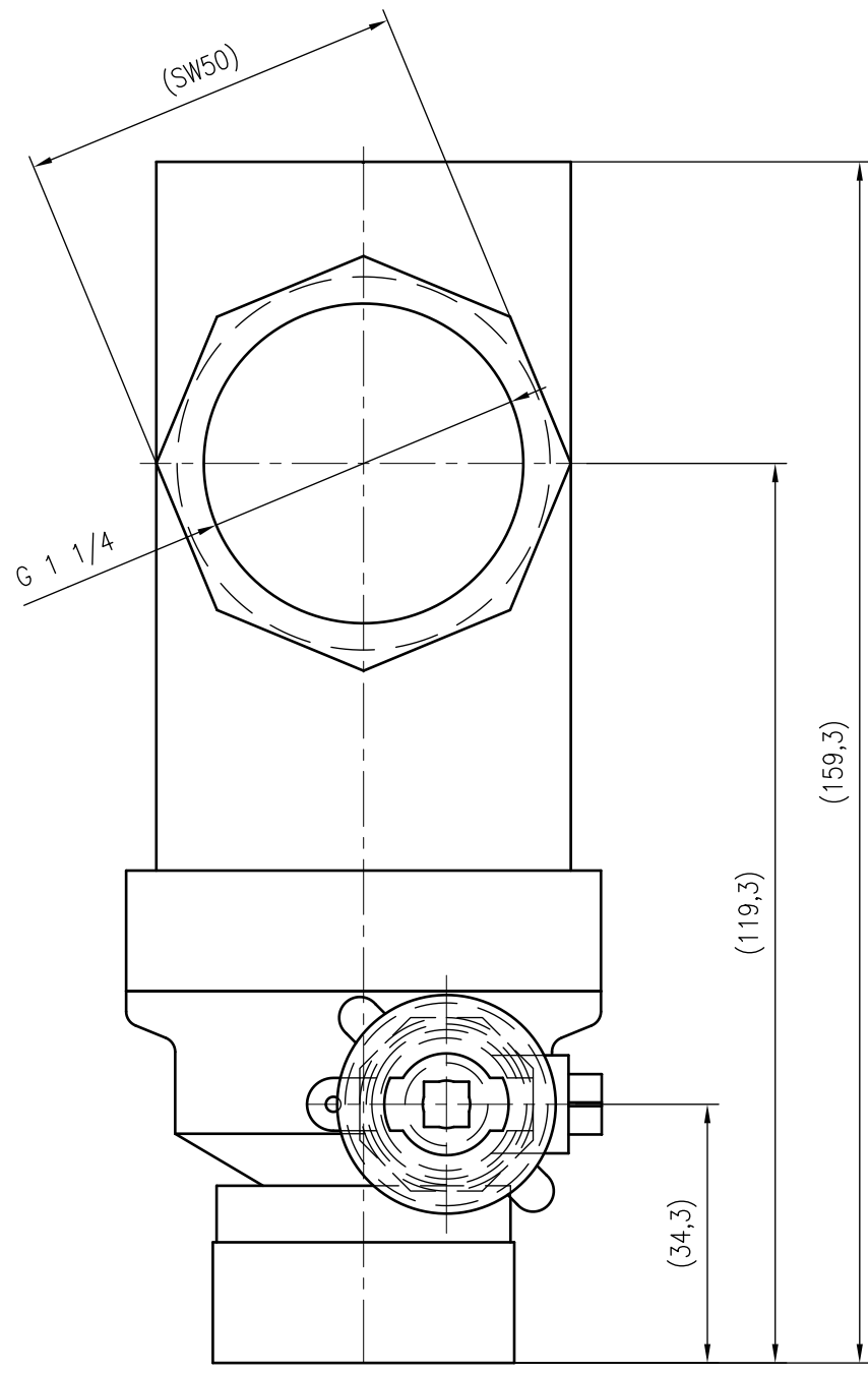
Side view
