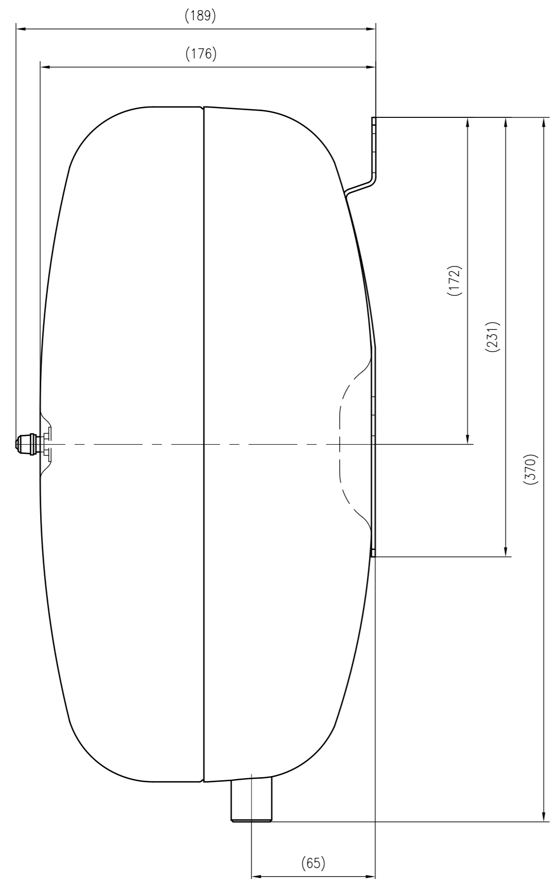
Side view
